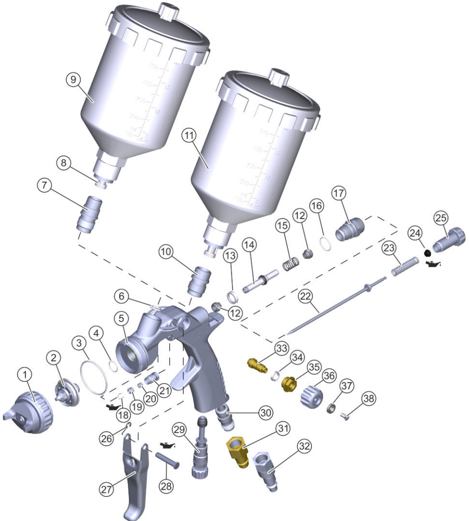
Fig. 25: Exploded view
