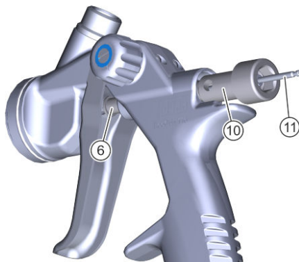
Fig. 19: Disassemble seal
